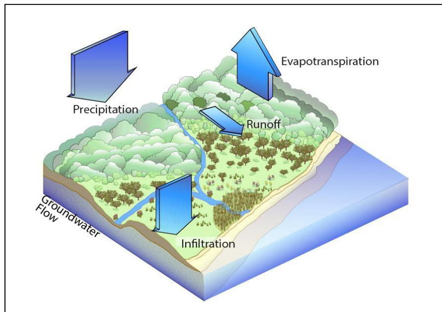
Figure C-1: Groundwater Recharge in the Hydrologic Cycle
